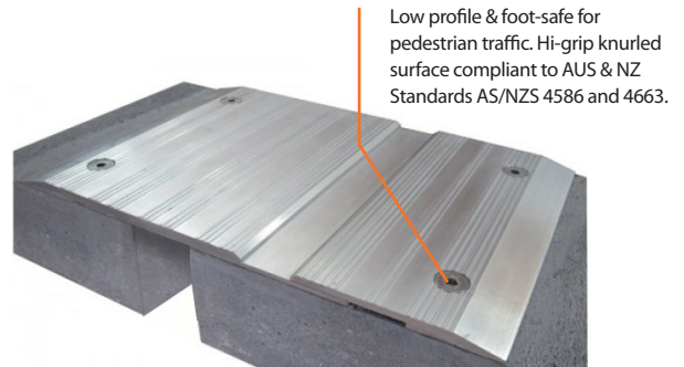
The SP Expansion Joint Cover System.
